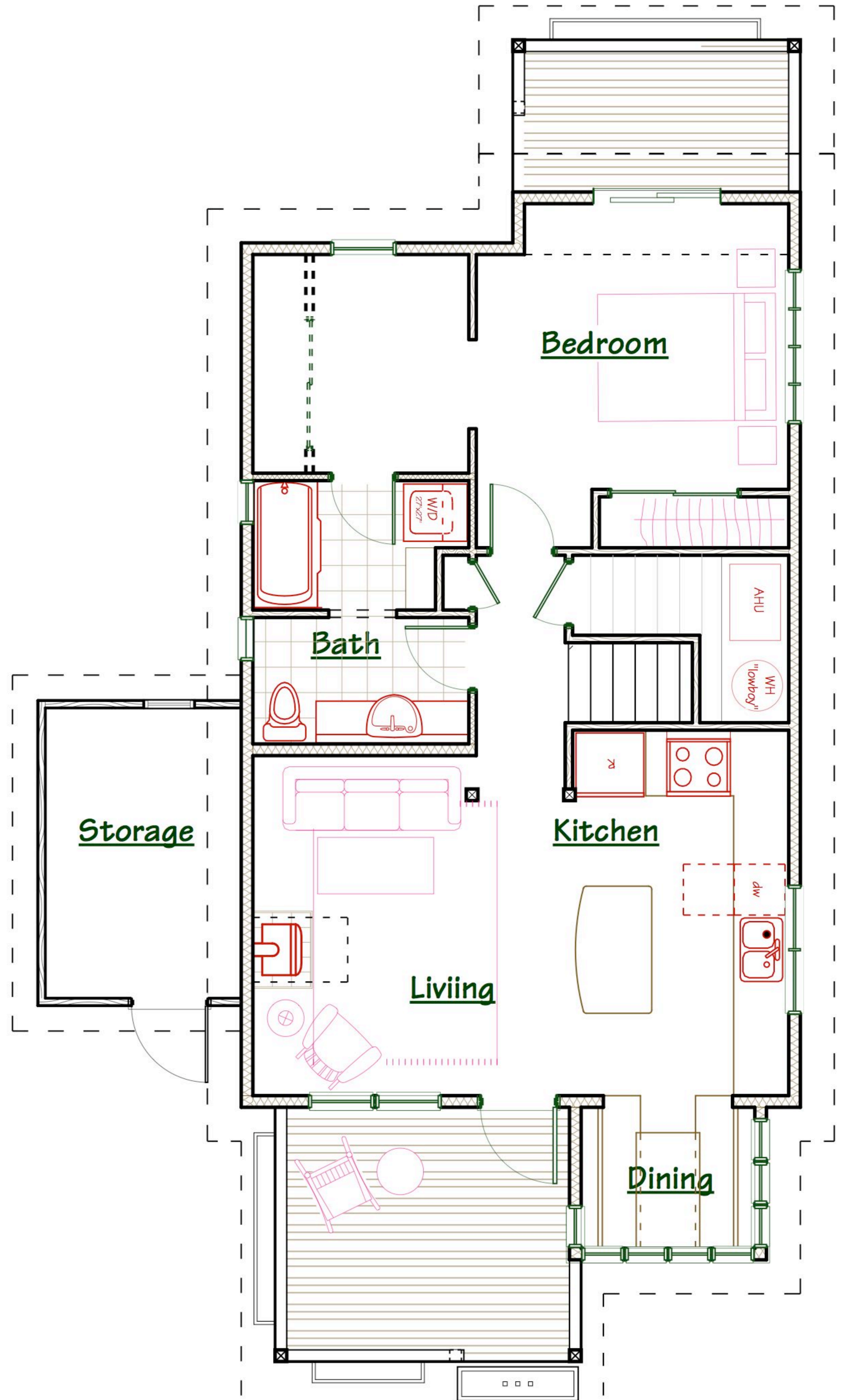
First Floor Plan
